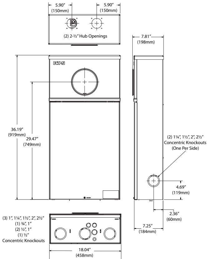
Metered, Service Entrance Rated ATS dimensions
